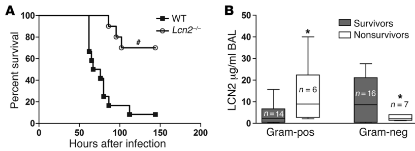
Figure 7 LCN2 is detrimental during pneumococcal pneumonia in mice and humans. (A) WT and Lcn2 -/- mice were infected with 4 \times 10^4 CFU S. pneumoniae and monitored for survival ( n = 12 per group). * P < 0.0001 versus WT (log-rank). (B) LCN2 levels in BAL of ICU patients with microbiologically confirmed bacterial pneumonia were analyzed according to the causative pathogen: Gram-positive ( n = 20 ) or Gram-negative ( n = 23 ) pneumonia. Data are expressed as box-and-whiskers plot. * P < 0.05 versus survivors ( t test).
