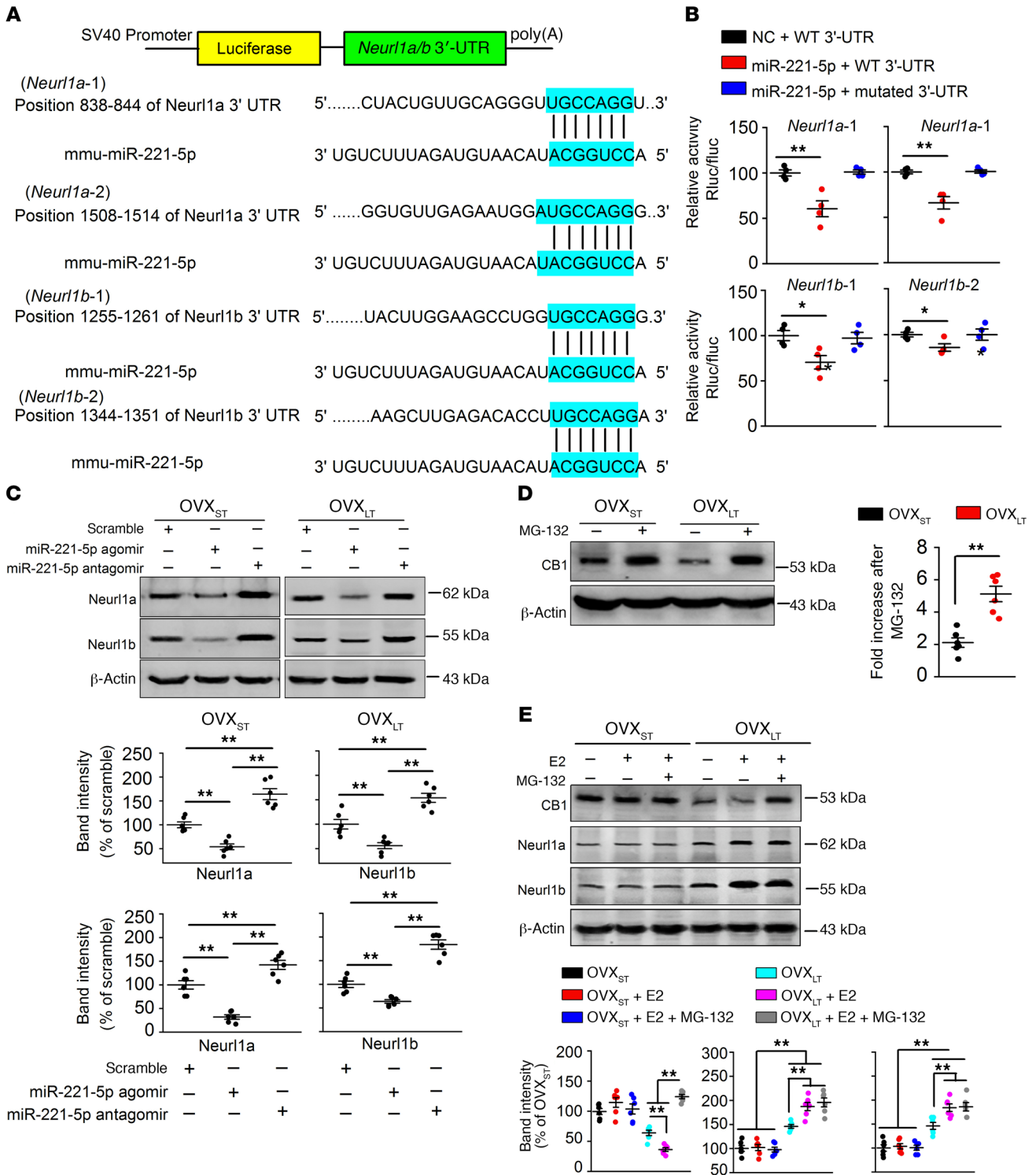
Figure 6. miR-221-5p regulating CB1 ubiquitination through Neur1a/b-dependent pathway. (A) Alignment of binding sequences for miR-221-5p in the 3'-UTRs of Neur1a and neur1b mRNAs. (B) Interaction between miR-221-5p and 3'-UTRs of Neur1a or neur1b mRNAs detected by luciferase reporter gene. n = 4 assays per group. *P < 0.05 , **P < 0.01 vs. negative control (NC) by 1-way ANOVA followed by Bonferroni's post hoc test. Rluc, renilla luciferase; Fluc, firefly luciferase. (C) mPFC injection of miR-221-5p agomir or antagonist regulated Neur1a and Neur1b expression in OVX ST and OVX LT mice. n = 6 mice per group. **P < 0.01 between the marked groups by 1-way ANOVA followed by Bonferroni's post hoc test. (D) MG-132 (a 26S proteasomal inhibitor, 5 mg/kg, 1 week, once daily, i.p.) induced a larger increase of CB1 level in OVX LT mice than that in OVX ST mice. n = 6 mice per group. **P < 0.01 by unpaired Student's t test. (E) E2-induced decrease of CB1 was blocked by MG-132 in OVX LT mice. E2 increased Neur1a and Neur1b levels in OVX LT mice, and higher Neur1a and Neur1b were found in OVX LT mice compared with OVX ST mice. n = 6 mice per group. **P < 0.01 between the marked groups by 2-way ANOVA followed by Bonferroni's post hoc test. Experimenters were not blinded to the treatment. Data are represented as mean \pm SEM.
